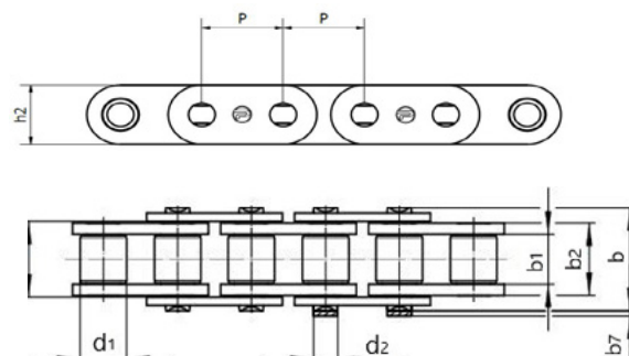
Straight side plates
