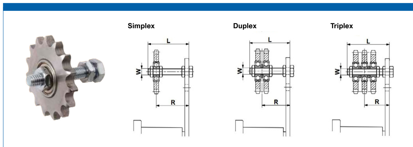
Sprocket wheel set type KS
