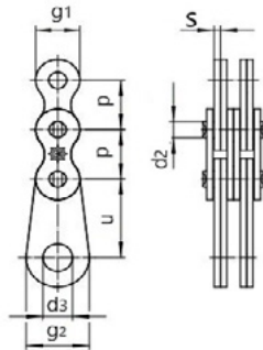
Inner end link
